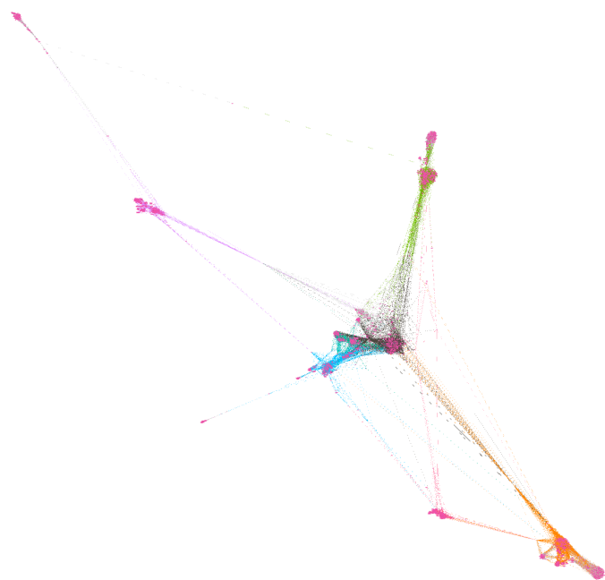
Force Atlas
